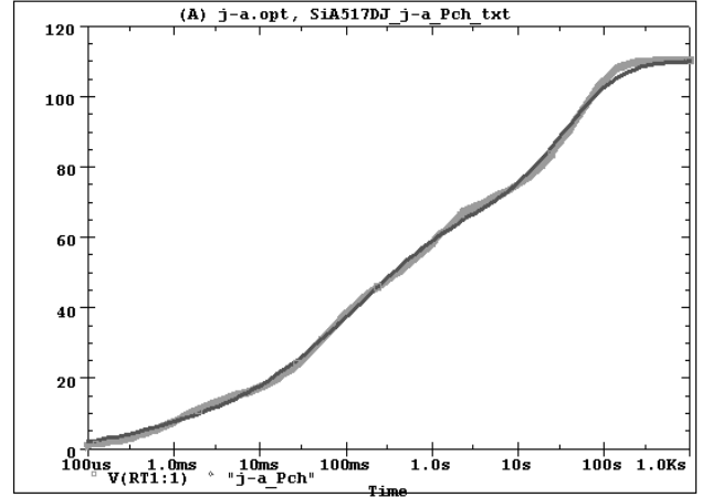
SiA517DJ Tank j-a P Channel Temperature:27.0
