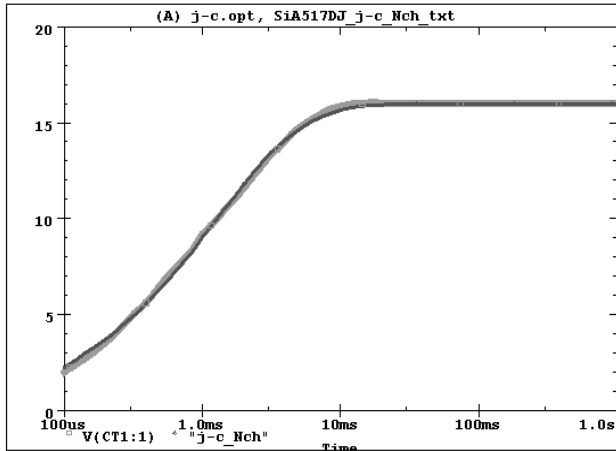
SiA517DJ Tank j-c N Channel Temperature:27.0
