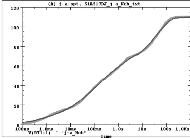
SiA517DJ Tank j-a N Channel Temperature:27.0
