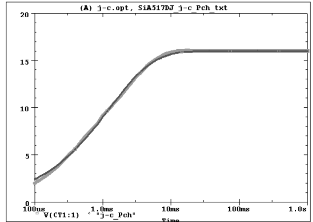
SiA517DJ Tank j-c P Channel Temperature:27.0
